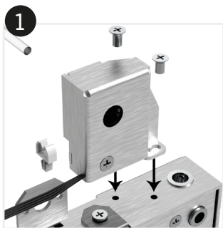
Fix the LED using the 2 screws
