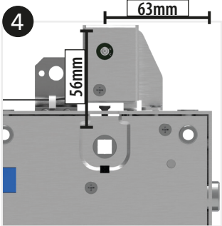
LED position quotas
